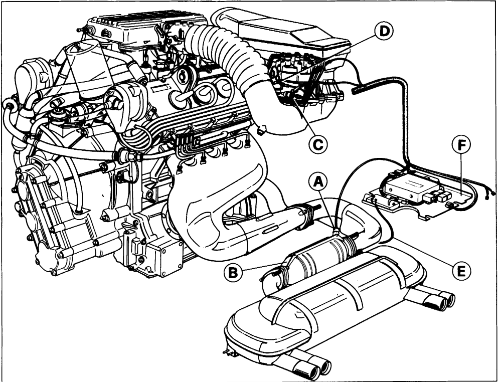
66) Oxygen sensor control system.
