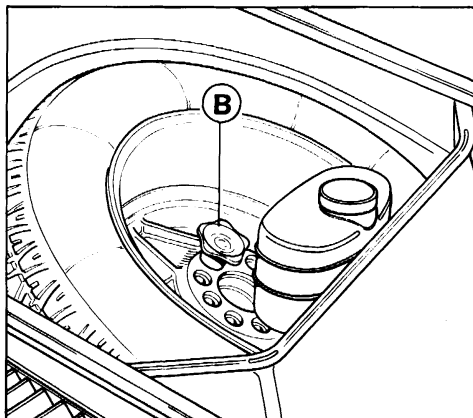
48) Location of spare wheel in boot. B - Spare wheel fixing nut.
