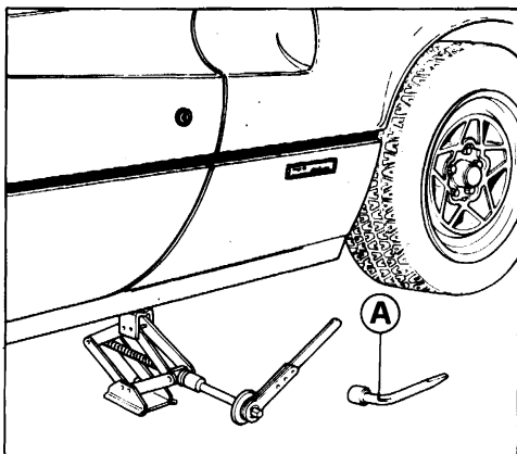
47) Jacking up the rear wheel.
